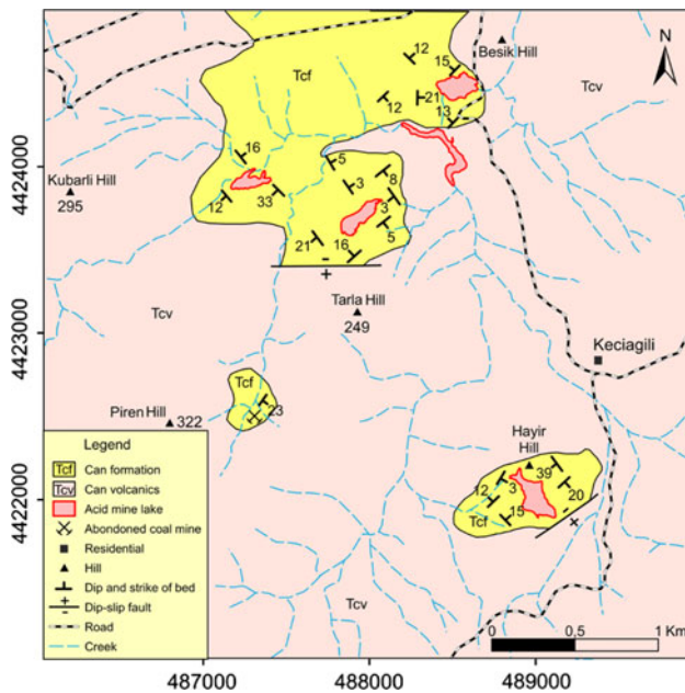
Fig. 4 Geological map of the study area
